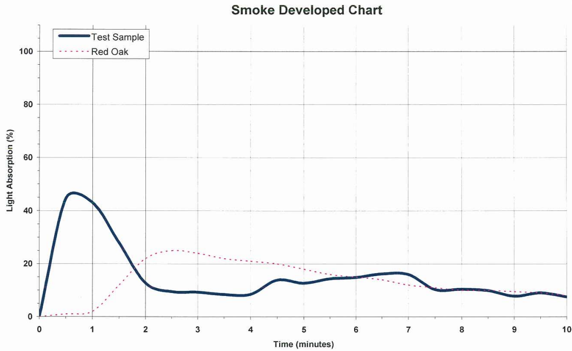
FIGURE 2. Smoke Developed
