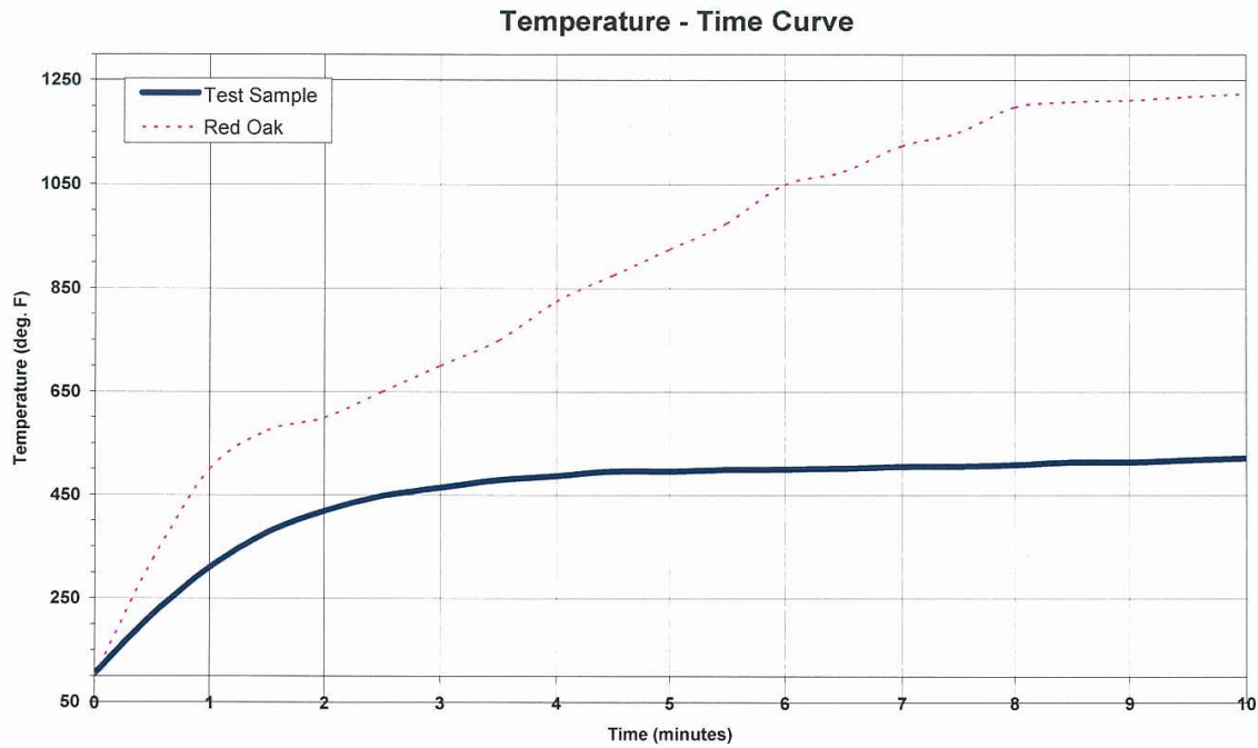
FIGURE 3. Temperature – 24 ft. Air Stream Thermocouple
