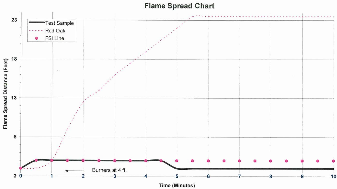
FIGURE 1. Flame Spread
